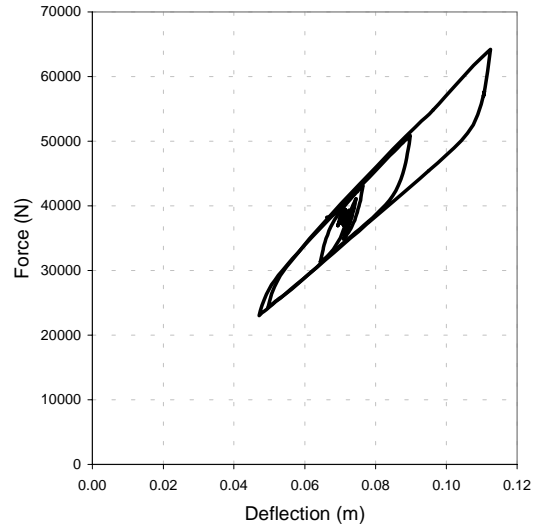
Figure 1(b) Characteristics of the quarter-truck multi-leaf steel spring used in this paper (typical).
