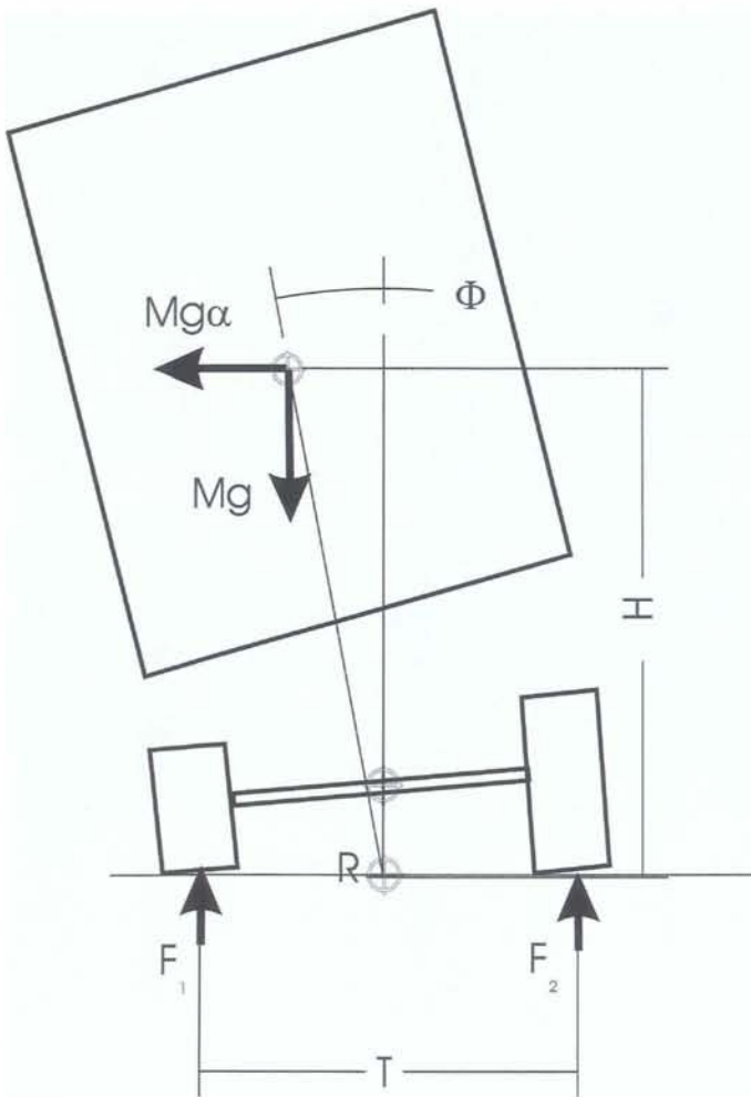
Figure 2 - Schematic showing heavy vehicle under lateral acceleration.
