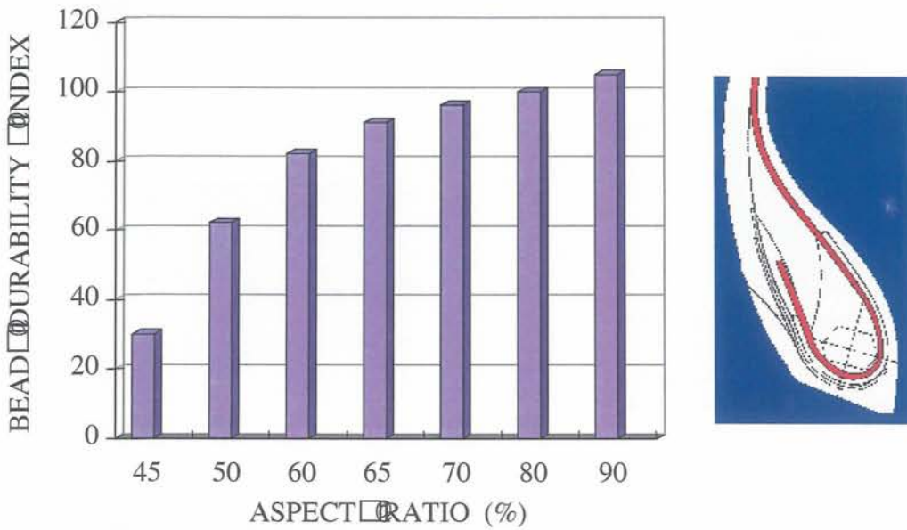
Figure 6 – Conventional bead structure, right, and trend of the durability as a function of the aspect ratio.
