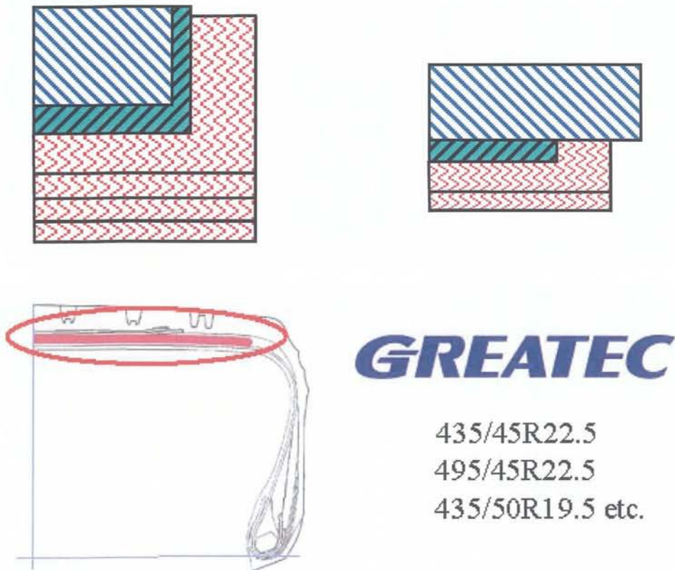
Figure 8 – Proposed belt package: the New WAVED belt.
