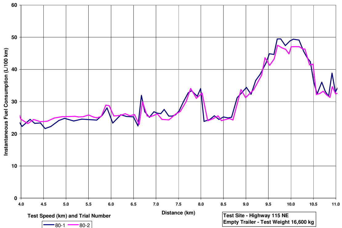
Figure 1 - Repeatability Curve
