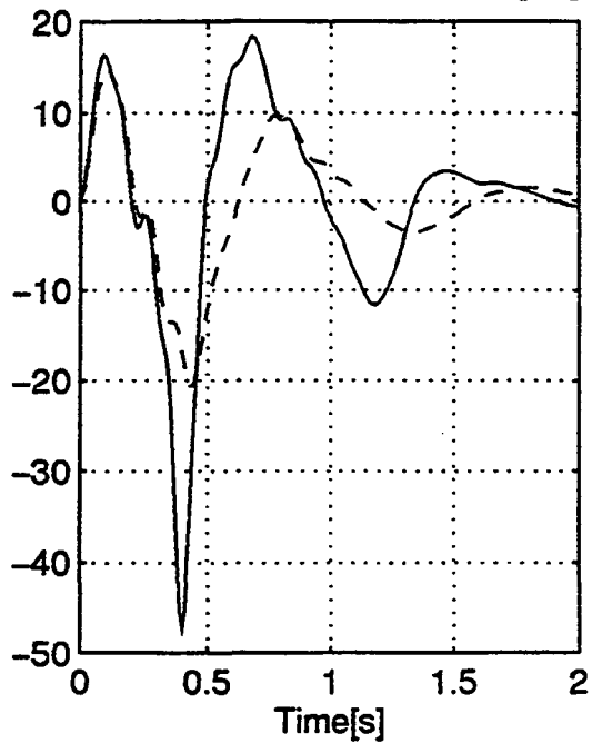
Figure 25. Dynamic wheel forces obtained when passing a 60 mm deep dip for two spring travels. [_____ 60 mm spring travel, ----- 130 mm spring travel].
