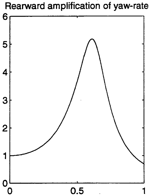
Figure 15. Truck and drawbar trailer, baseline. Rearward amplification of yaw velocity vs frequency.
