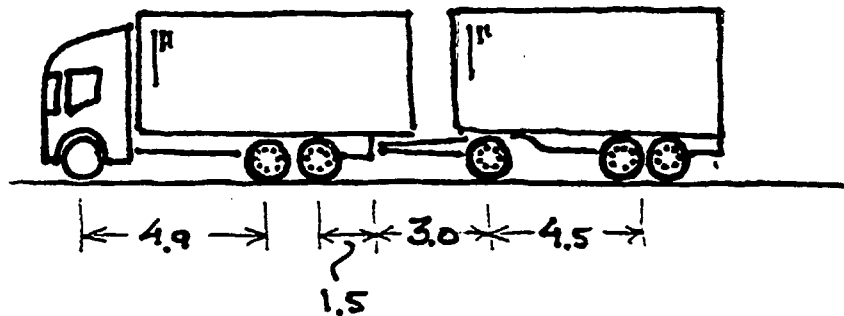
Figure 28. Truck and drawbar trailer. GCW = 44 t.
