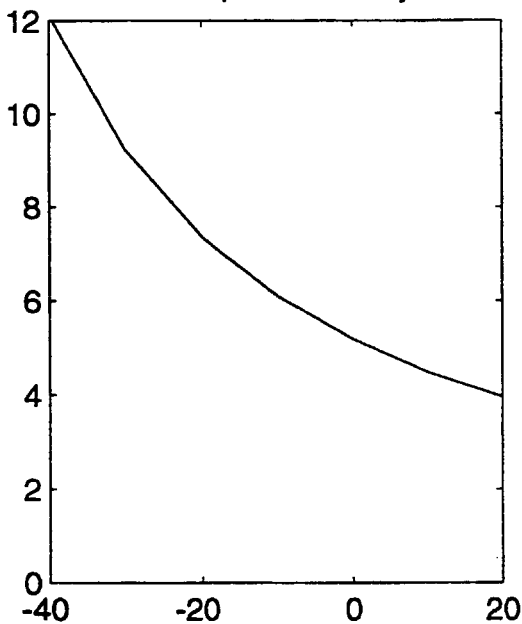
Figure 19. Truck and drawbar trailer. Influence of changes [%] of the cornering stiffness of trailer tyres.
