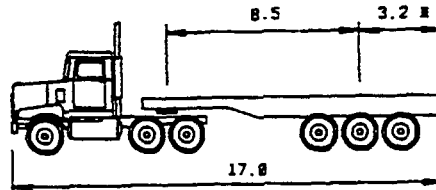
Truck and Semi-trailer (Articulated vehicle)
