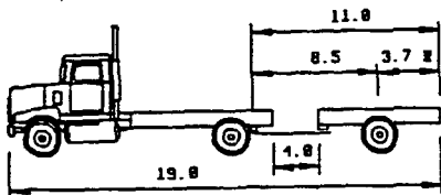
Truck and Simple Trailer (one axle set trailer)
