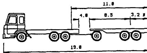
Truck and Full Trailer (two axle set trailer)
