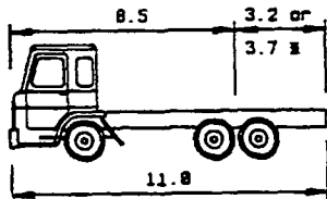
Rigid Truck
