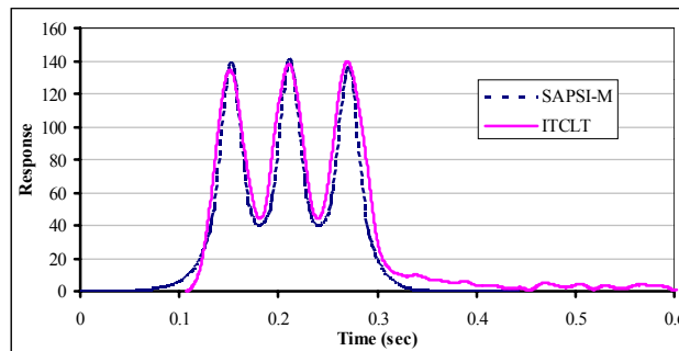
Figure 1. Typical Response Pulses from SAPMSI-M and ITCLT Test Results.
