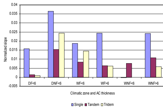
b) Normalized slope vs. axle configurations
