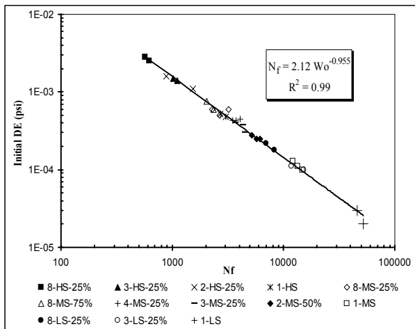
Figure 2. Fatigue curve based on dissipated energy density.
