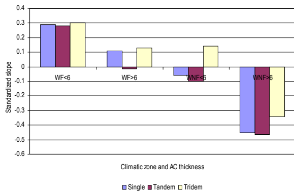
(a) Standardized slope vs. axle configurations
