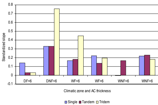
a) Standardized slope vs. axle configurations
