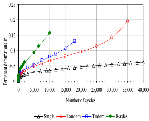
(a) Cumulative vertical deformation vs. number of cycles for different axle configurations-High stress level
