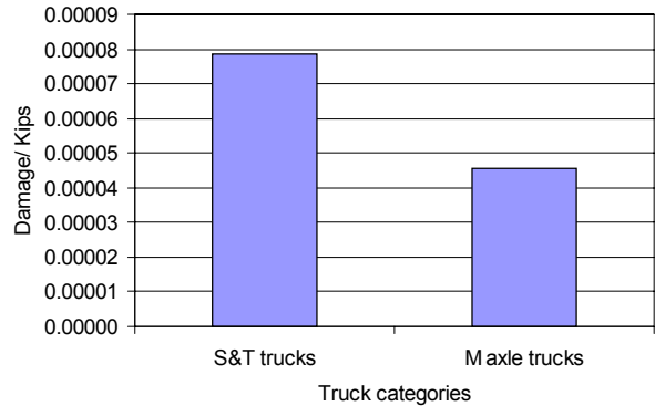
(f) Normalized damage vs. truck categories
