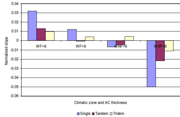
(b) Normalized slope vs. axle configurations
