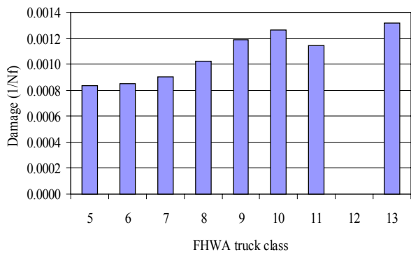
(c) Damage vs. FHWA truck classes
