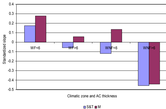
(c) Standardized slope vs. truck configurations
