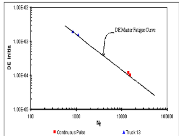
Figure 3. Fatigue response from continuous load pulse and truck no. 13.
