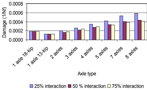
(a) Damage vs. axle configurations
