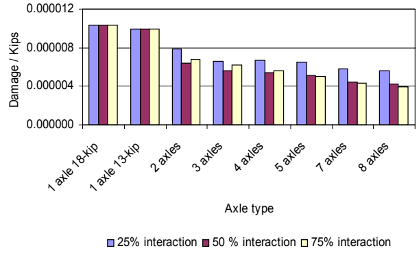
(b) Normalized damage vs. axle configurations
