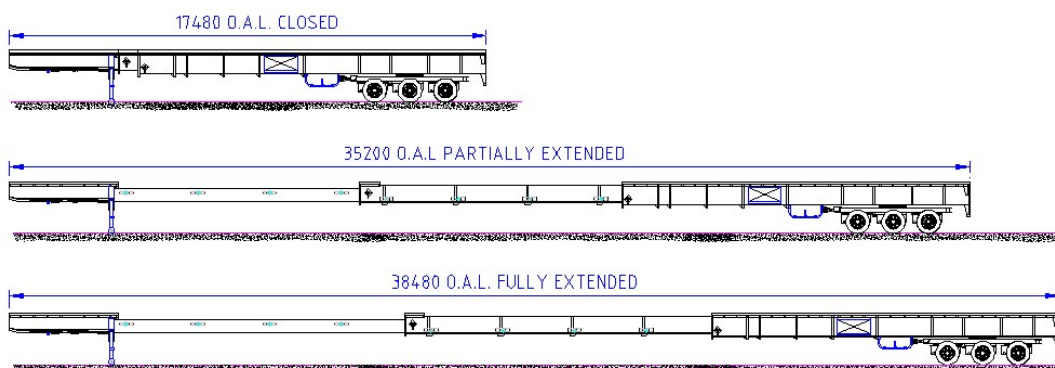
Figure 1 – Innovative steerable extendable semi-trailer.
