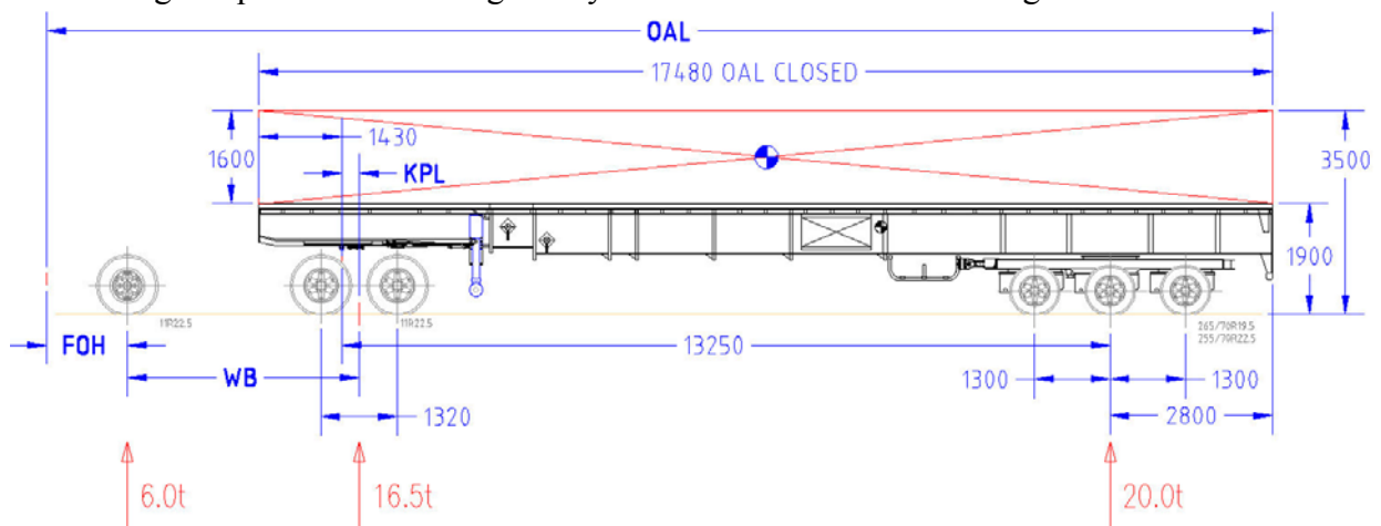
Figure 3 – Dimensions of the innovative steerable extendable semi-trailer
