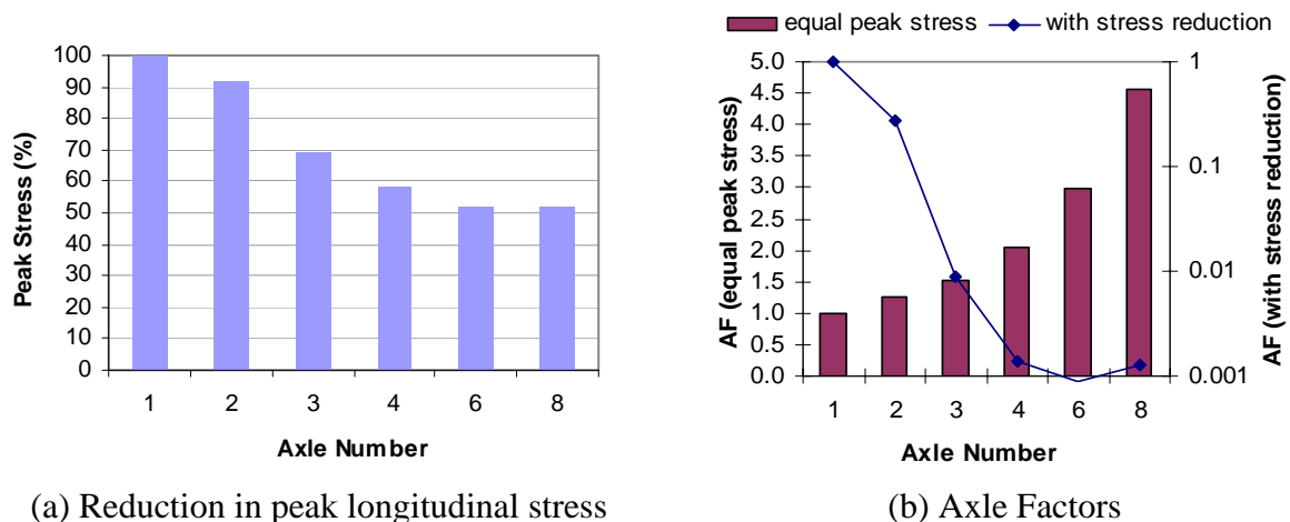
Figure 3 –Axle factors taking into account stress reduction
