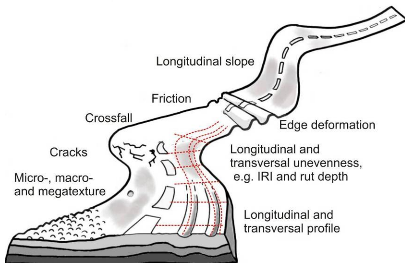
Figure 2 – Example of periodic road data used as support to pavement management systems
